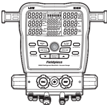
4 Port Model SM482V
